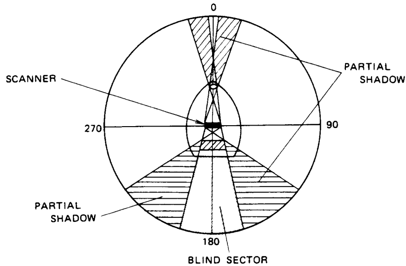
FIG. 2-10 SHADOWS
