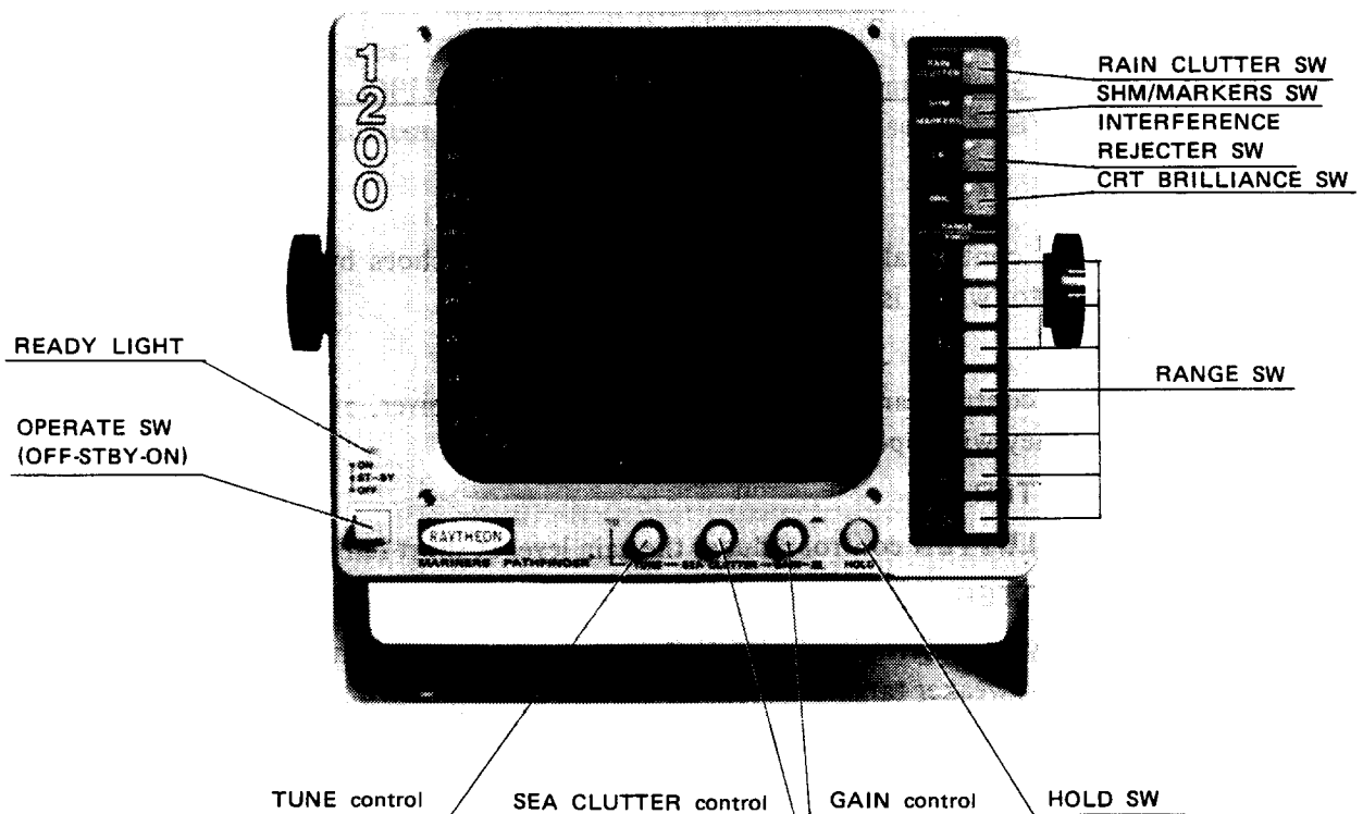
FIG. 2-1 OPERATING CONTROLS
