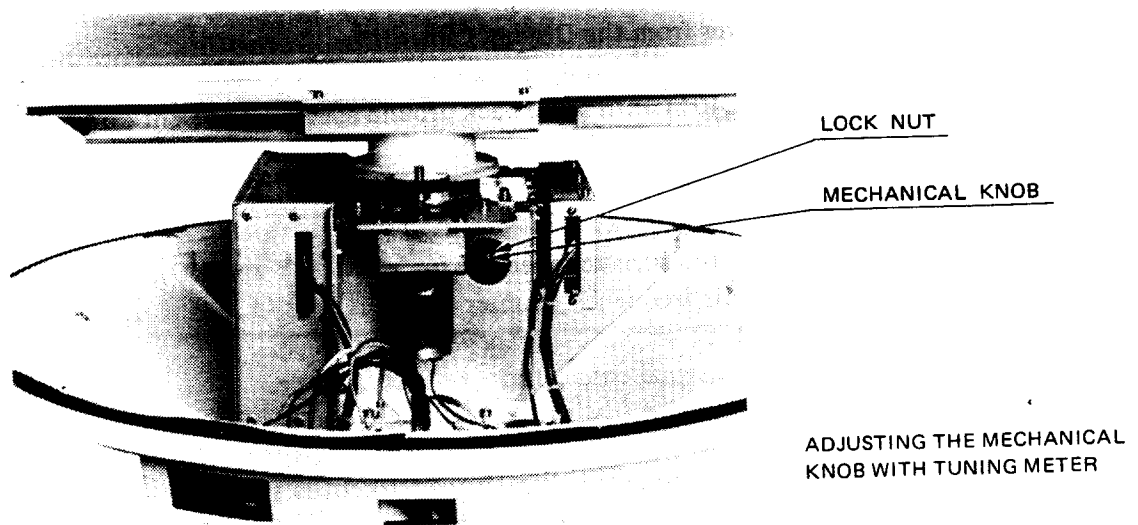
Fig. 5-1 GUNN OSCILLATOR TUNING
