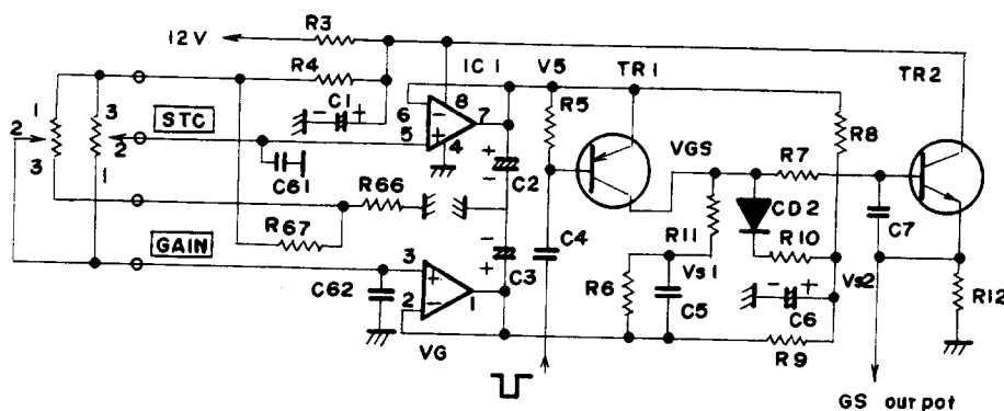
FIG. 6-7 GAIN - STC CIRCUIT
