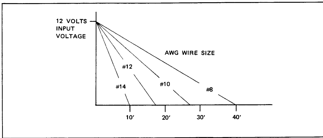
POWER CABLE LENGTH TABLE 4-1 POWER CABLE SIZE VERSUS LENGTH
