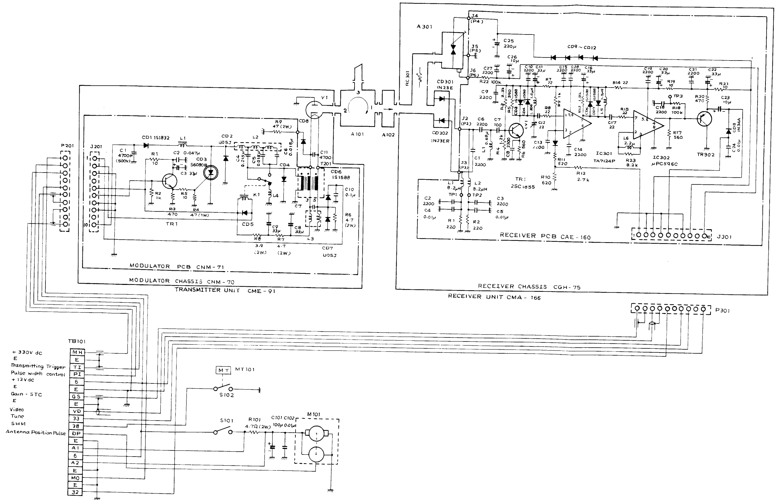
FIG. 107 CIRCUIT DRAWING OF M89362 SCANNER UNIT
