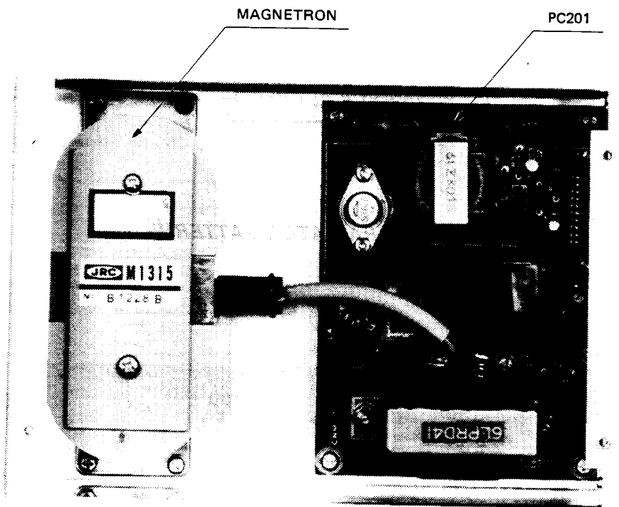
FIG. 6-3 TRANSMITTER UNIT
