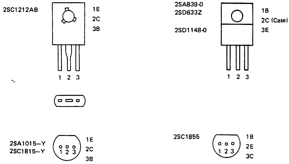
FIG. 5-7 IDENTIFICATION OF TRANSISTOR LEADS
